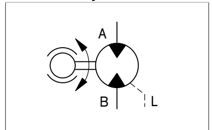
Motor with dynamic brake
