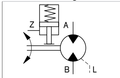
Motor with holding brake
